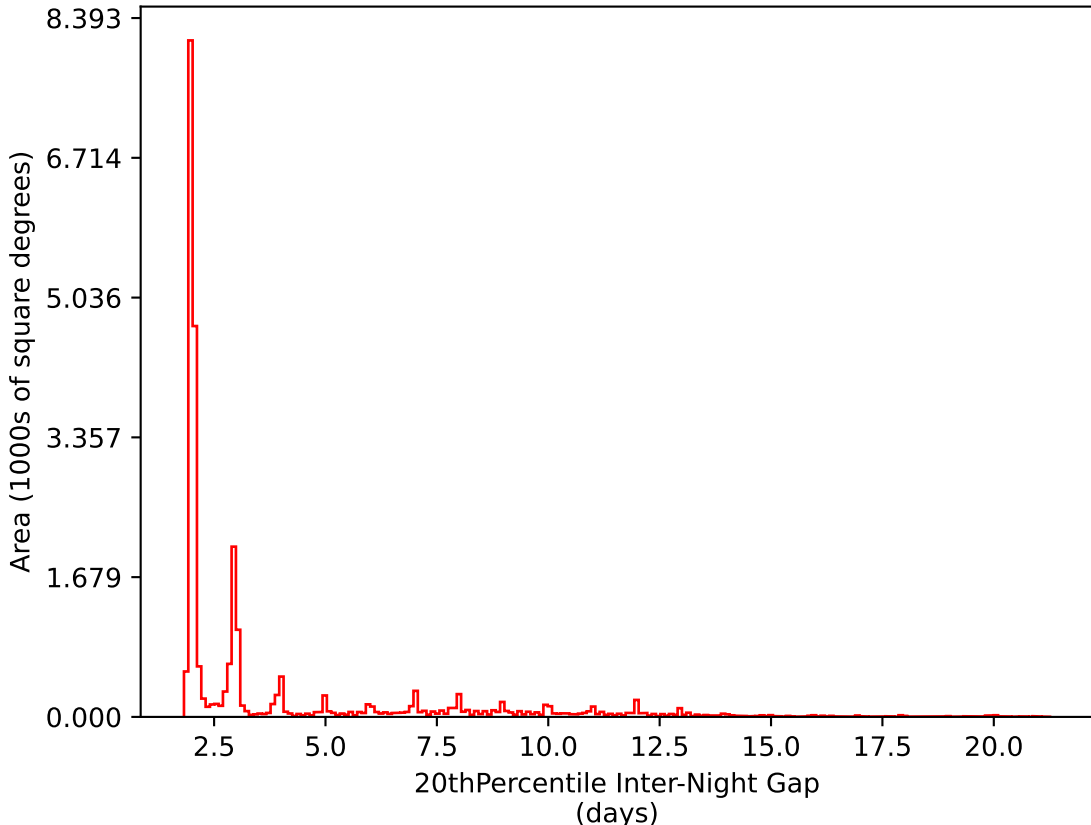
too_elab_r128_d3_gz_v3.4_10yrs All sky i band: 20thPercentile Inter-Night Gap
