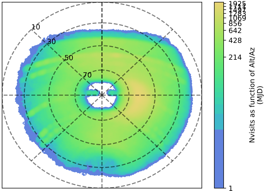
too_elab_r128_d3_gz_v3.4_10yrs y: Nvisits as function of Alt/Az
