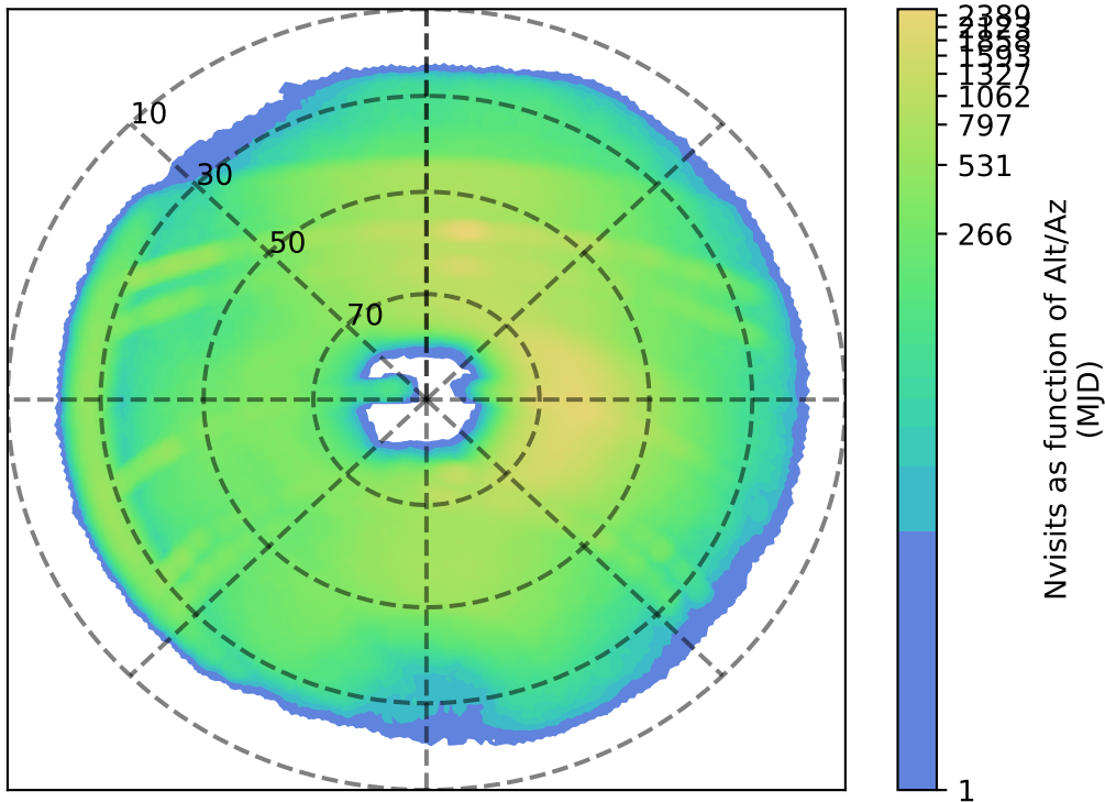
too_elab_r128_d3_gz_v3.4_10yrs r: Nvisits as function of Alt/Az
