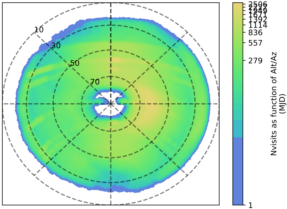
too_elab_r128_d3_gz_v3.4_10yrs i: Nvisits as function of Alt/Az
