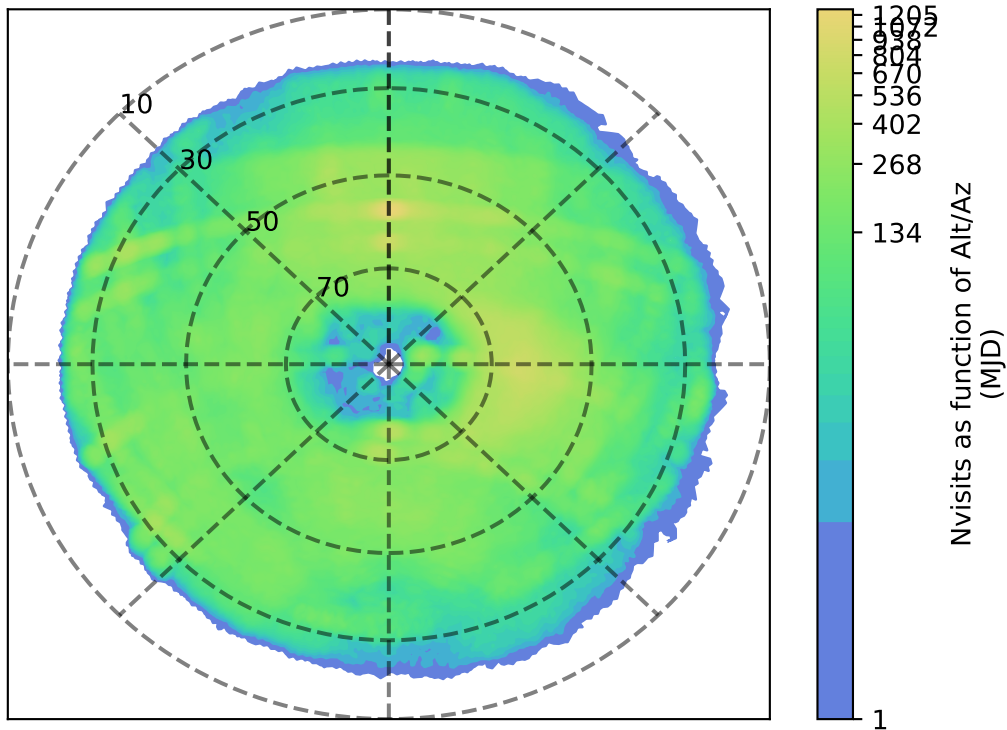
too_elab_r128_d3_gz_v3.4_10yrs g: Nvisits as function of Alt/Az
