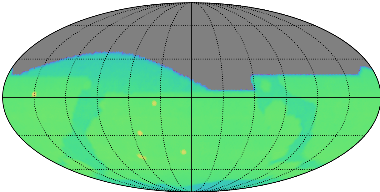
too_elab_r128_d3_gz_v3.4_10yrs : CoaddM5
