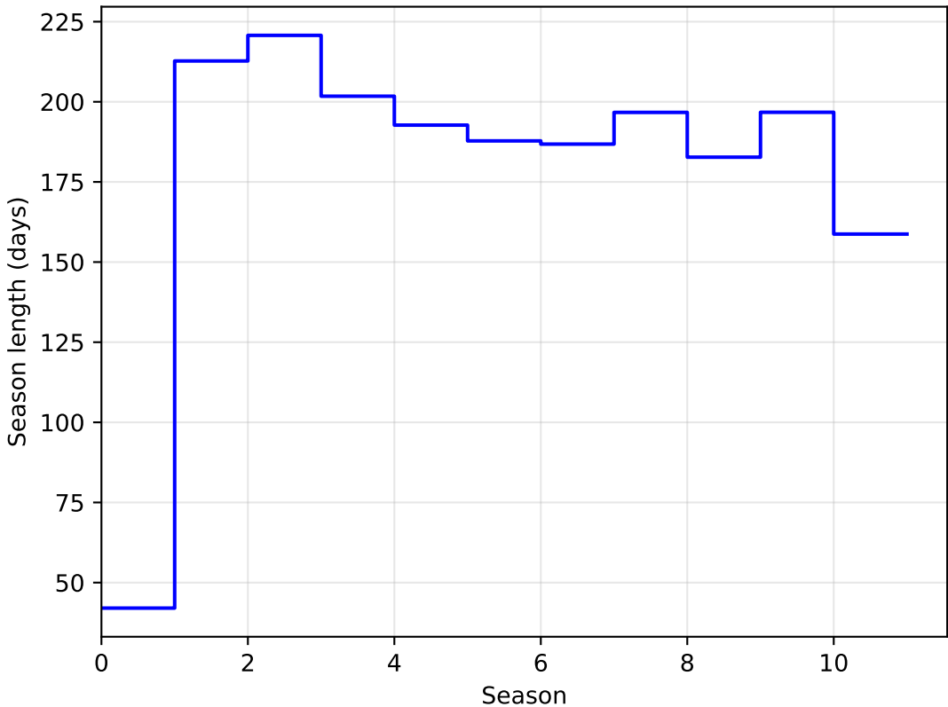
too_elab_r128_d3_gz_v3.4_10yrs DD: COSMOS all bands: SeasonLength
