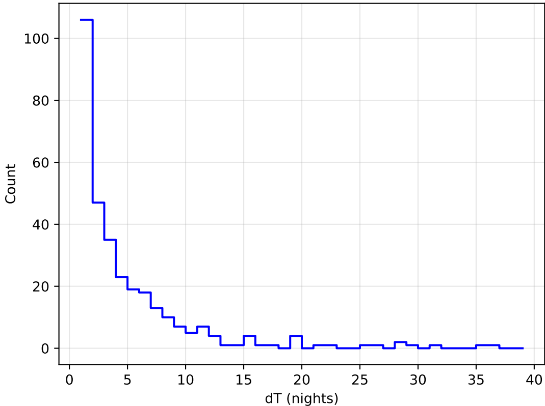
too_elab_r128_d3_gz_v3.4_10yrs all bands: DD:WFD Delta Nights Histogram
