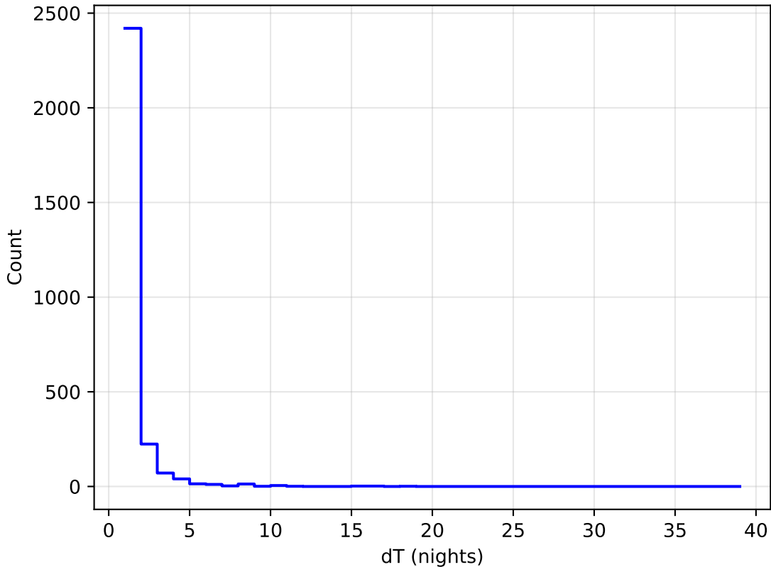
too_elab_r128_d3_gz_v3.4_10yrs all bands: DD:WFD Delta Nights Histogram
