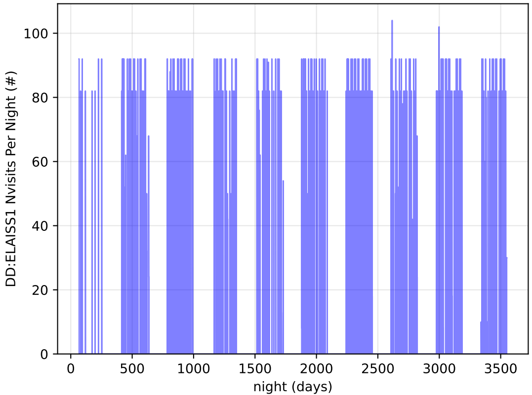
too_elab_r128_d3_gz_v3.4_10yrs all bands: DD:ELAISS1 Nvisits Per Night
