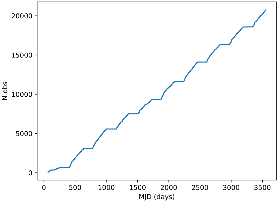
too_elab_r128_d3_gz_v3.4_10yrs all bands: DD:ELAISS1 Cumulative NVisits
