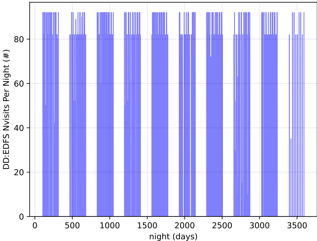
too_elab_r128_d3_gz_v3.4_10yrs all bands: DD:EDFS Nvisits Per Night
