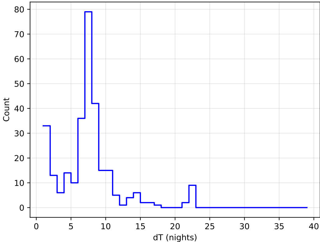
too_elab_r128_d3_gz_v3.4_10yrs all bands: DD:EDFS Delta Nights Histogram
