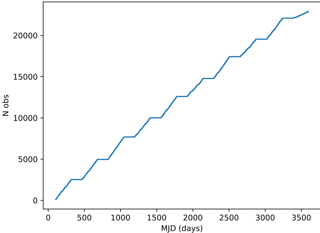
too_elab_r128_d3_gz_v3.4_10yrs all bands: DD:EDFS Cumulative NVisits
