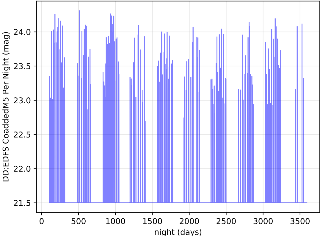
too_elab_r128_d3_gz_v3.4_10yrs y band: DD:EDFS CoaddedM5 Per Night
