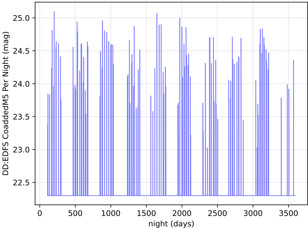
too_elab_r128_d3_gz_v3.4_10yrs u band: DD:EDFS CoaddedM5 Per Night
