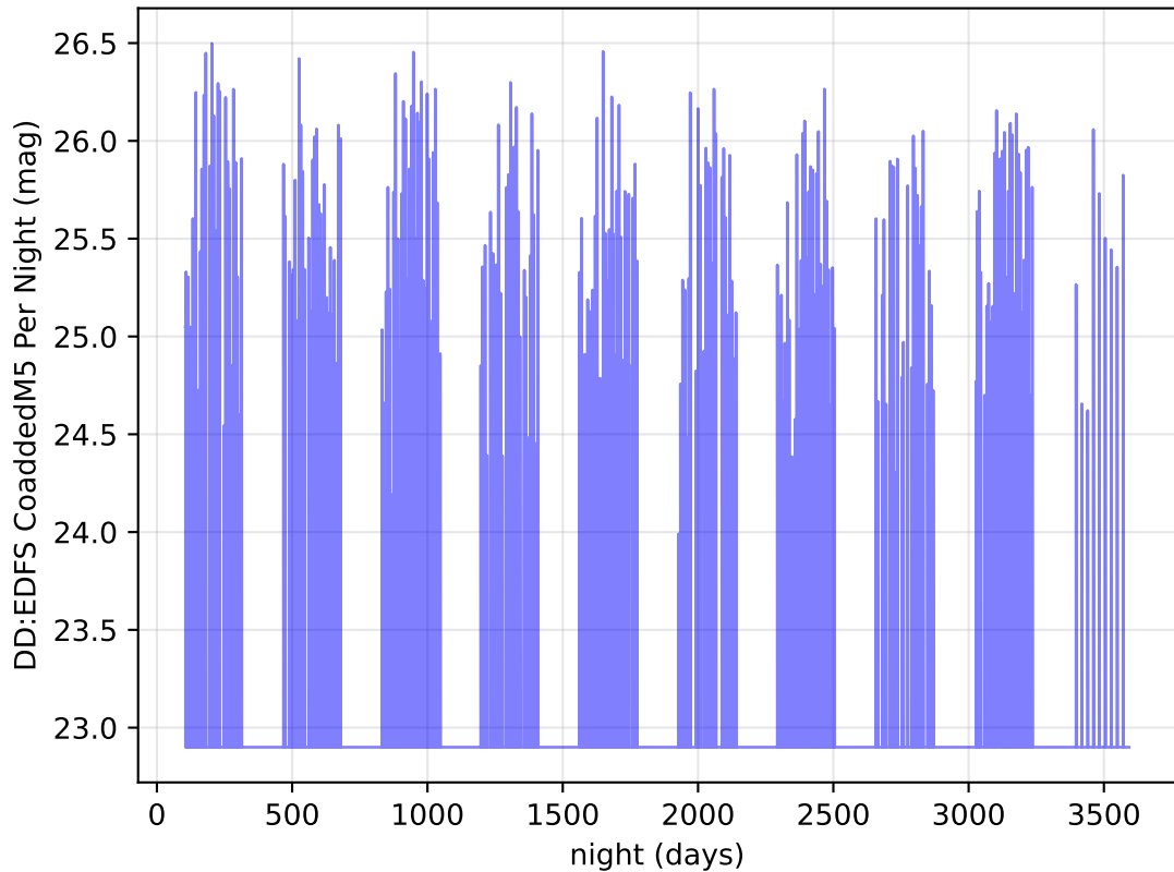
too_elab_r128_d3_gz_v3.4_10yrs r band: DD:EDFS CoaddedM5 Per Night
