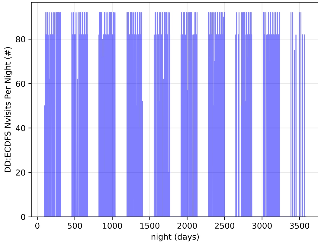
too_elab_r128_d3_gz_v3.4_10yrs all bands: DD:ECDFS Nvisits Per Night
