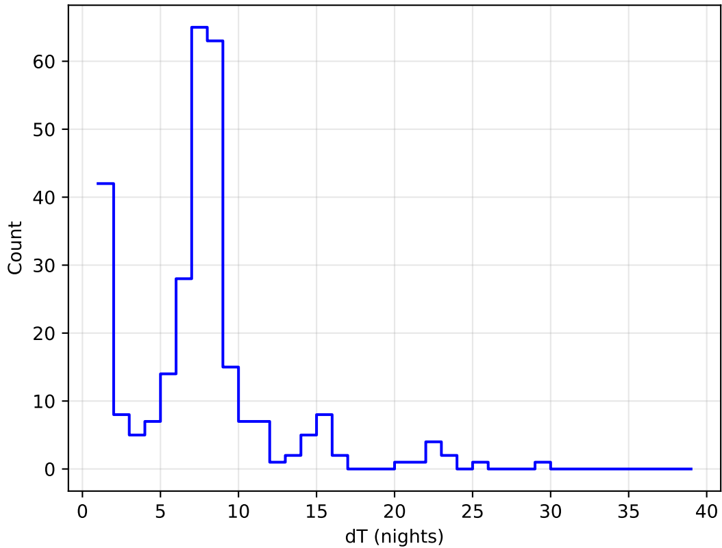
too_elab_r128_d3_gz_v3.4_10yrs all bands: DD:ECDFS Delta Nights Histogram
