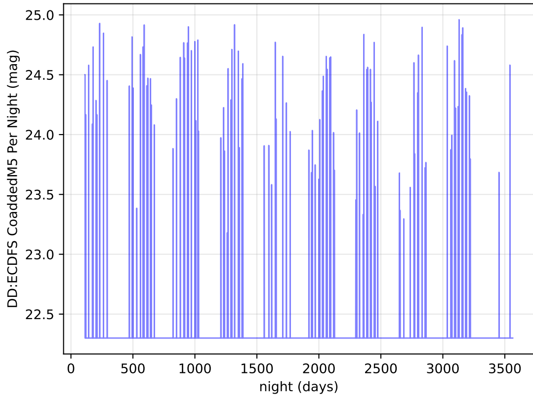
too_elab_r128_d3_gz_v3.4_10yrs u band: DD:ECDFS CoaddedM5 Per Night
