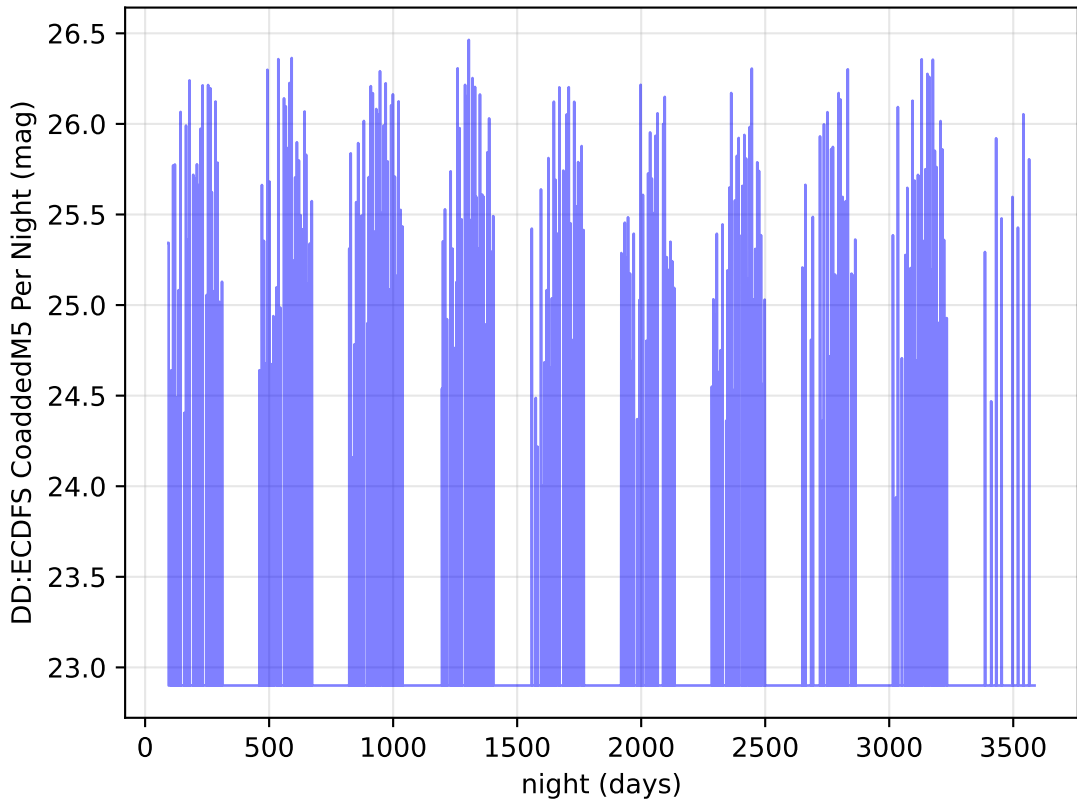
too_elab_r128_d3_gz_v3.4_10yrs r band: DD:ECDFS CoaddedM5 Per Night
