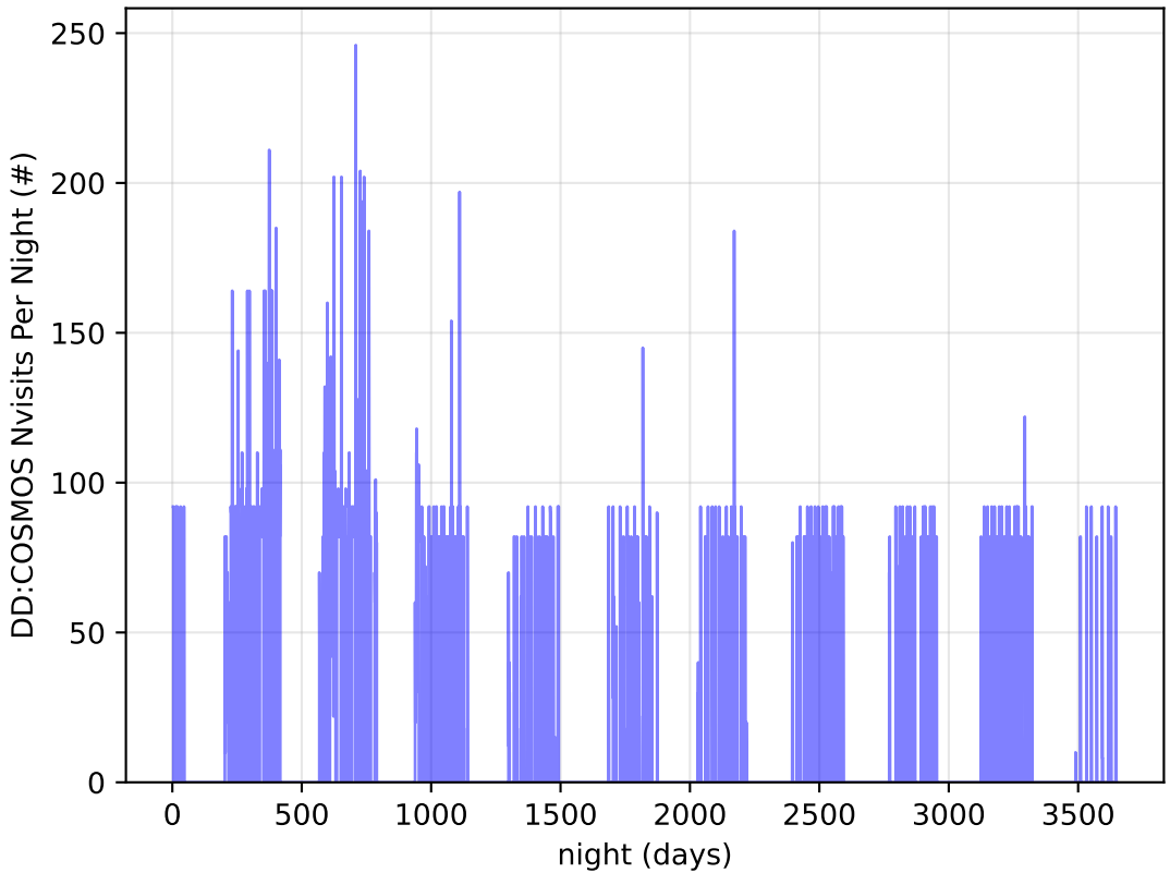
too_elab_r128_d3_gz_v3.4_10yrs all bands: DD: COSMOS Nvisits Per Night
