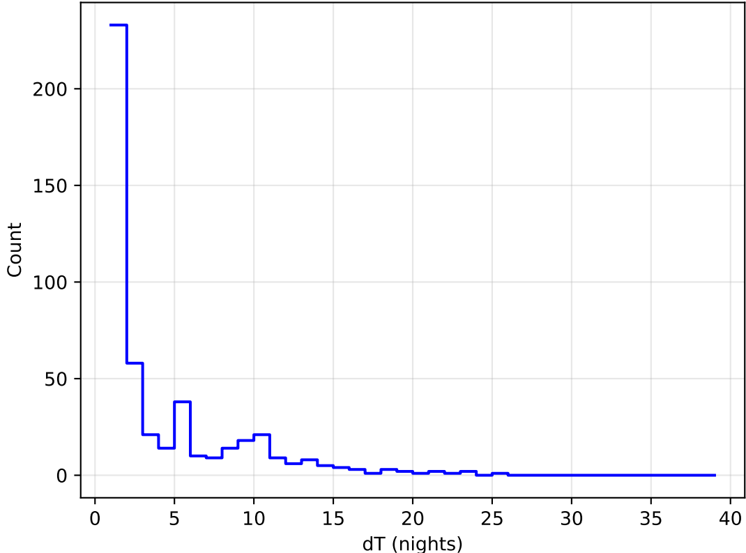
too_elab_r128_d3_gz_v3.4_10yrs all bands: DD: COSMOS Delta Nights Histogram
