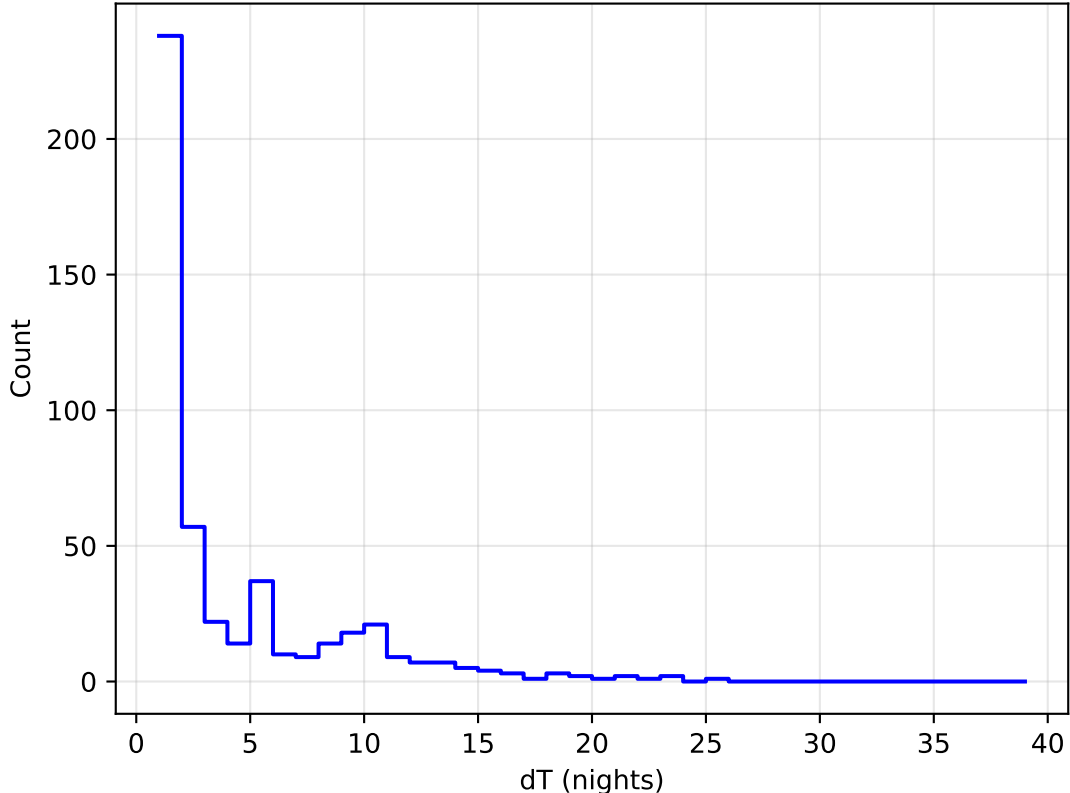
too_elab_r128_d3_gz_v3.4_10yrs all bands: DD:COSMOS Delta Nights Histogram
