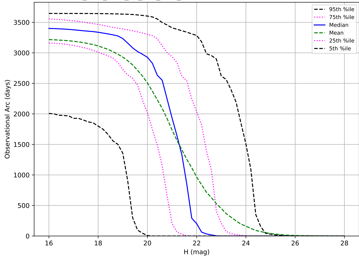
too_elab_r128_d3_griz_v3.4_10yrs: Observational Arc Length PHA
