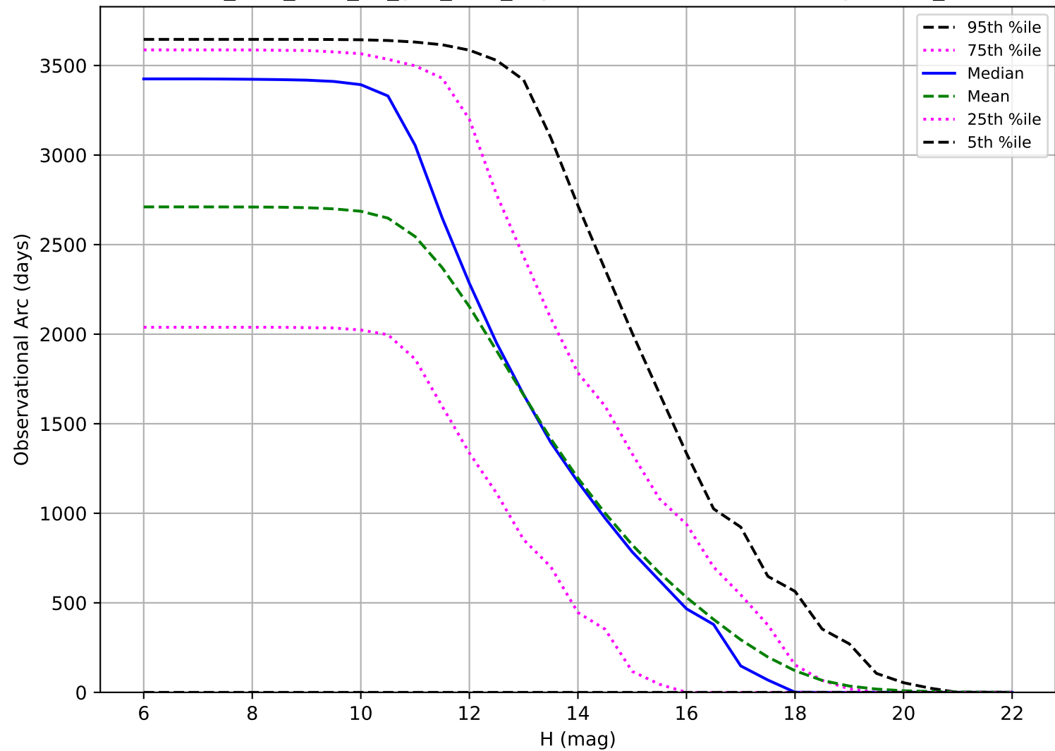
too_elab_r128_d3_griz_v3.4_10yrs: Observational Arc Length OCC_r5
