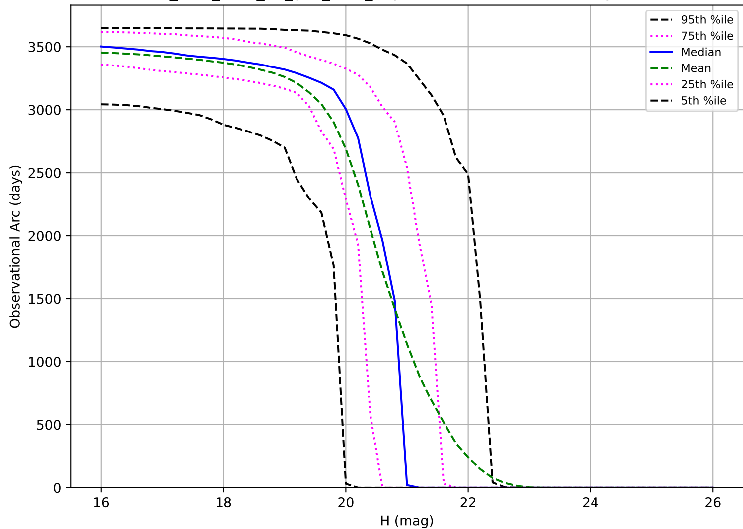
too_elab_r128_d3_griz_v3.4_10yrs: Observational Arc Length MBA
