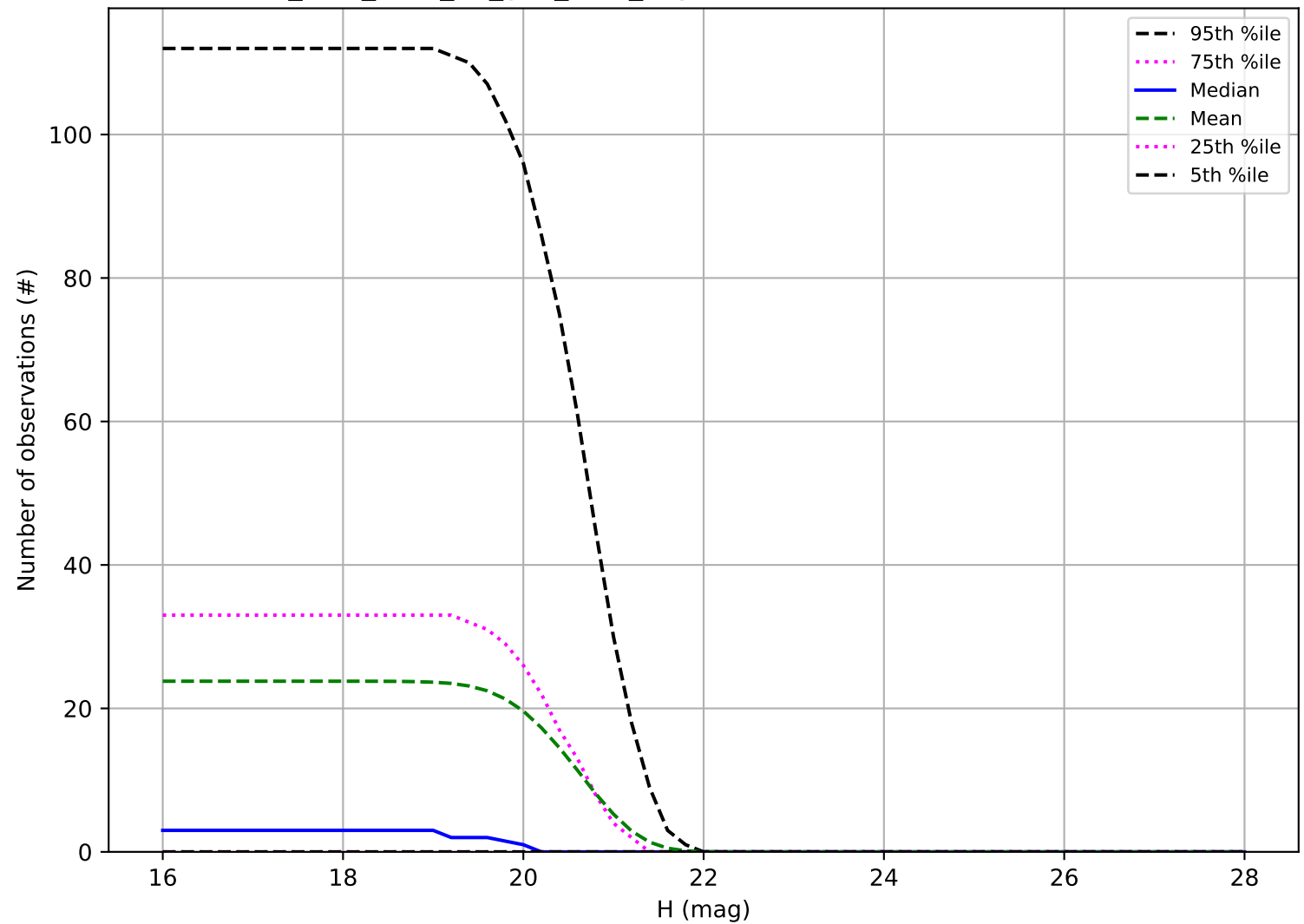
too_elab_r128_d3_griz_v3.4_10yrs: Number of observations Vatira
