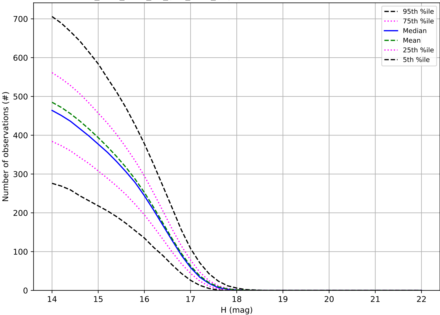
too_elab_r128_d3_griz_v3.4_10yrs: Number of observations Trojan
