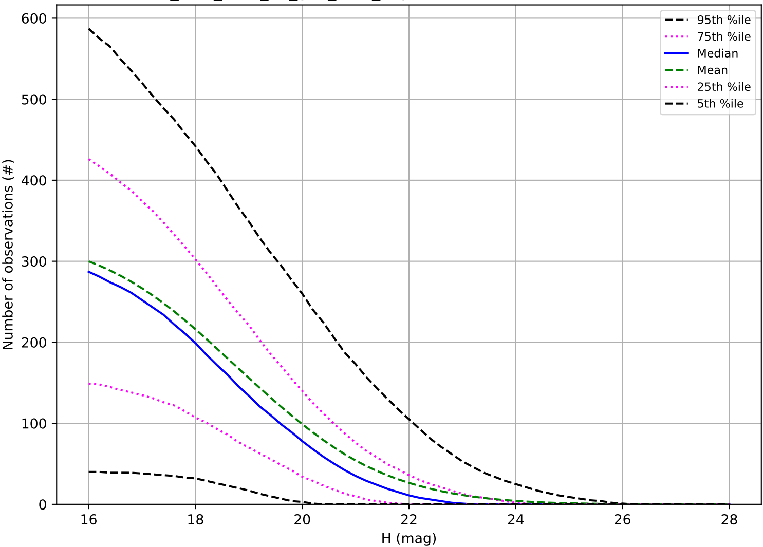
too_elab_r128_d3_griz_v3.4_10yrs: Number of observations PHA
