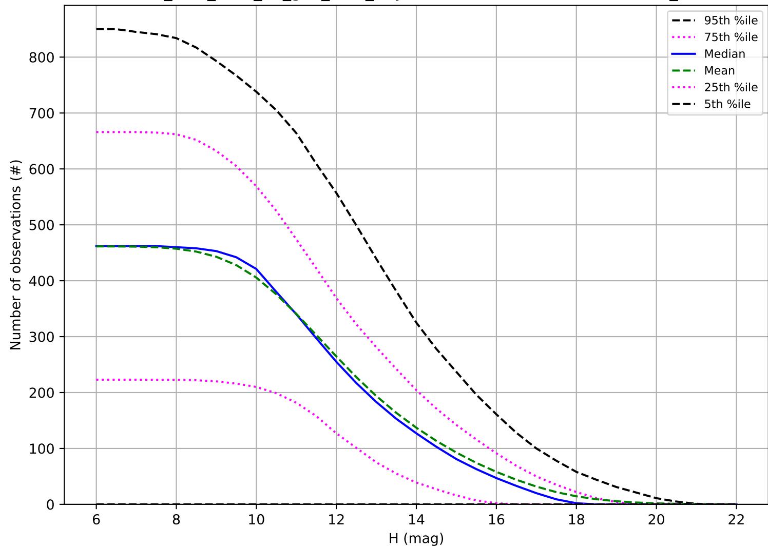
too_elab_r128_d3_griz_v3.4_10yrs: Number of observations OCC_r5
