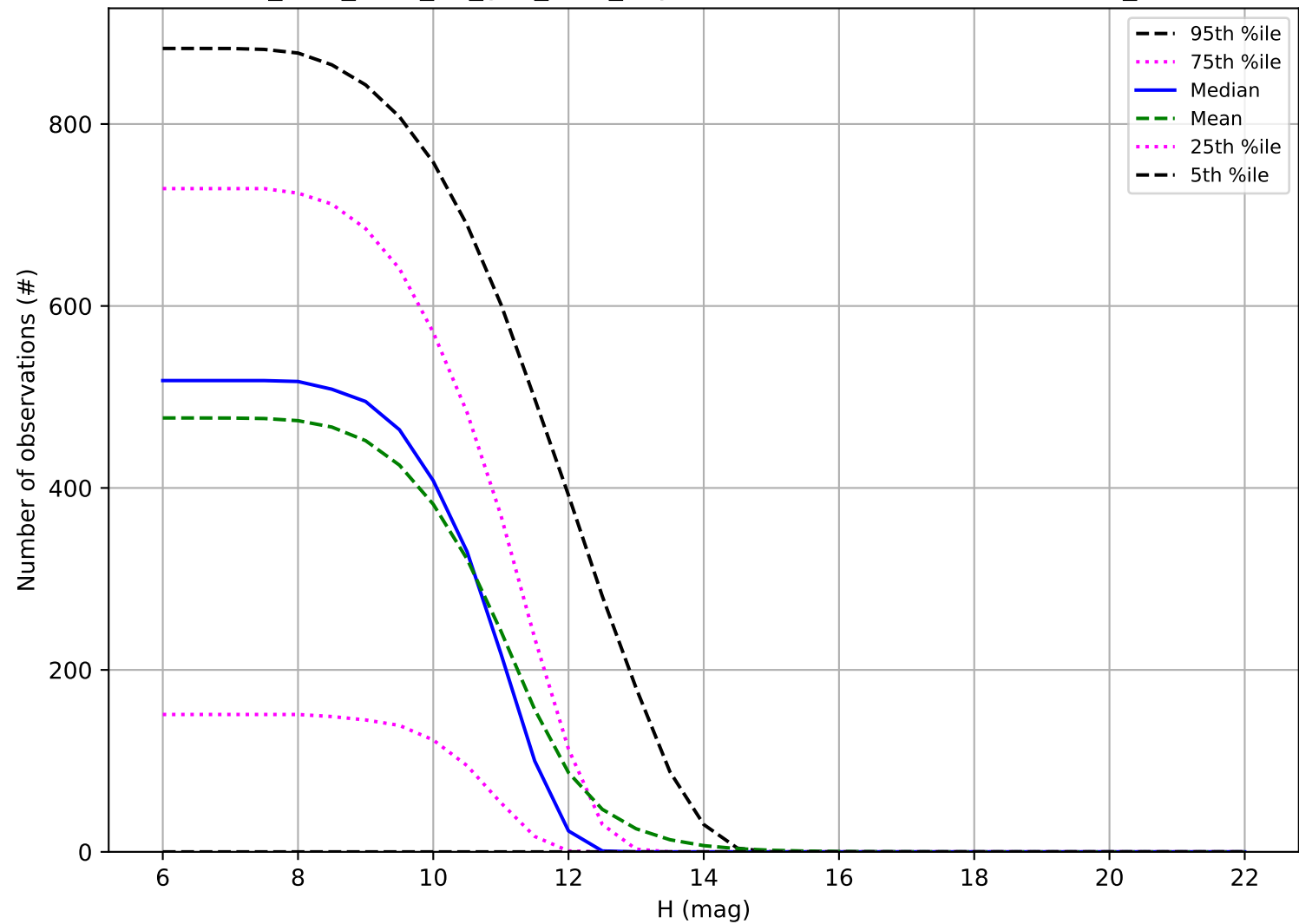
too_elab_r128_d3_griz_v3.4_10yrs: Number of observations OCC_r20
