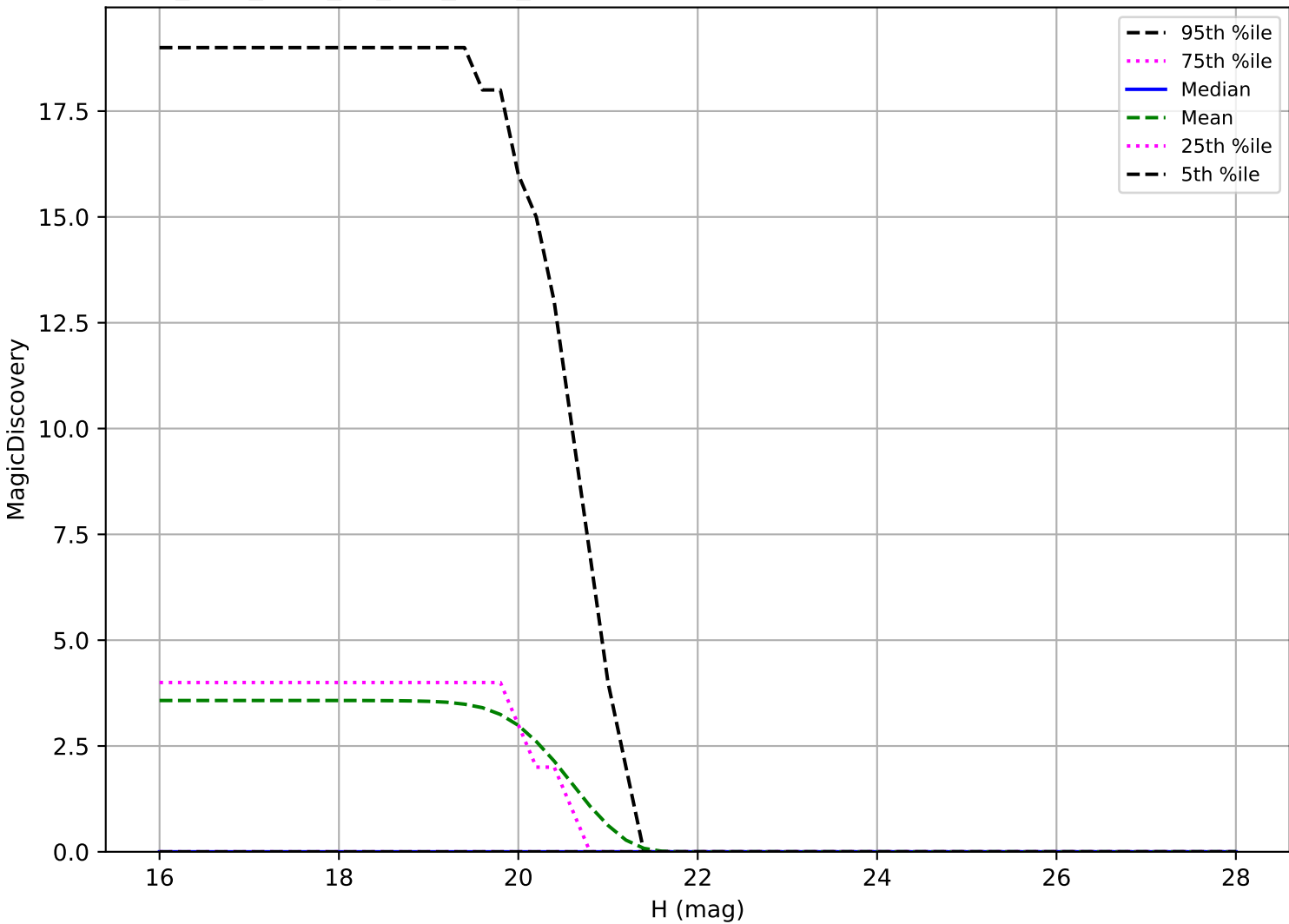
too_elab_r128_d3_griz_v3.4_10yrs: Vatira 6 detections in 60 nights detection loss
