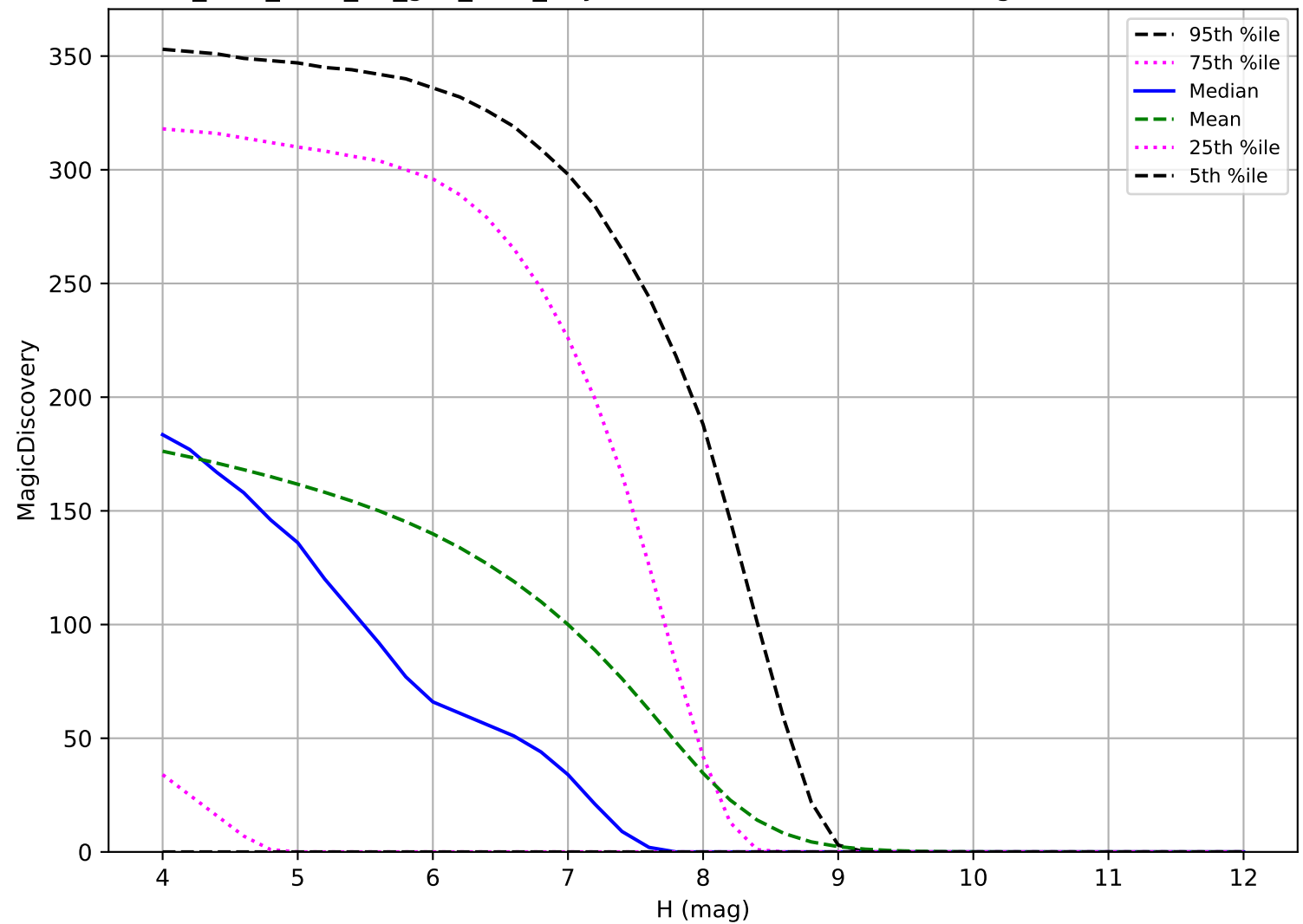
too_elab_r128_d3_griz_v3.4_10yrs: TNO 6 detections in 60 nights detection loss
