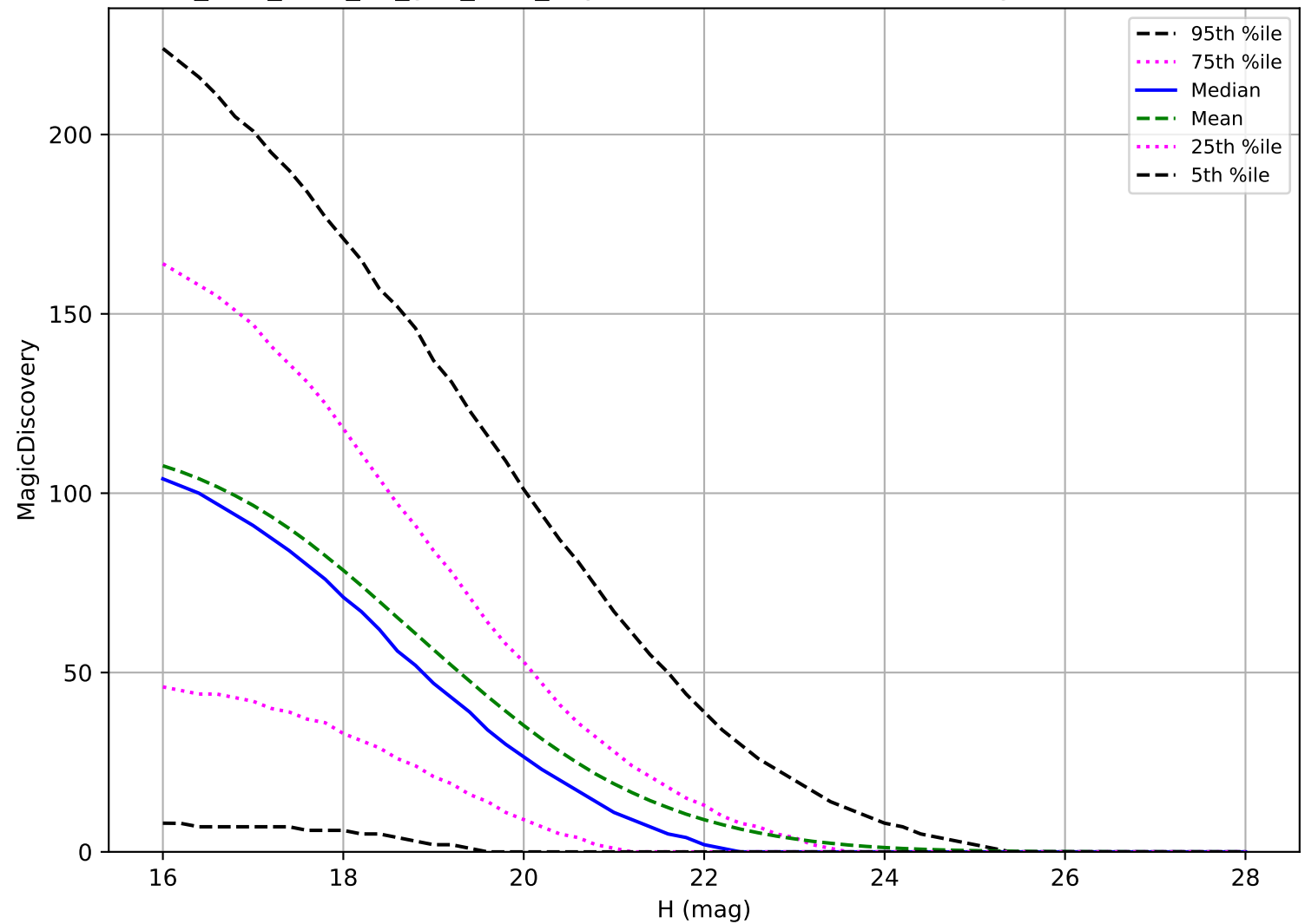
too_elab_r128_d3_griz_v3.4_10yrs: PHA 6 detections in 60 nights detection loss
