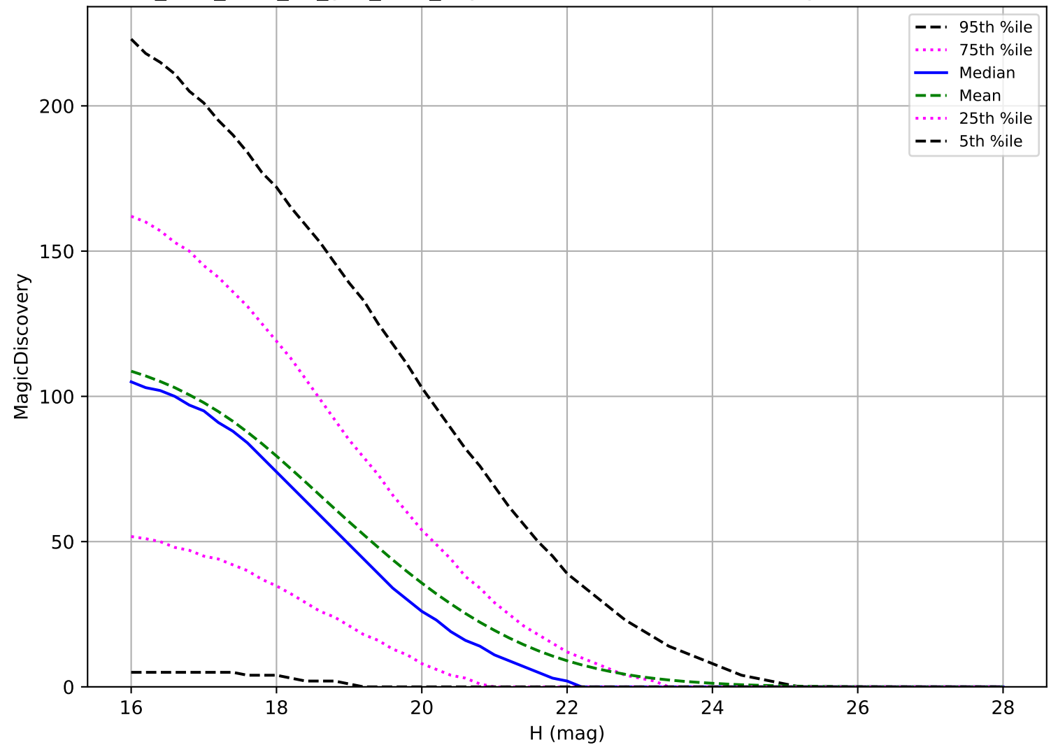
too_elab_r128_d3_griz_v3.4_10yrs: NEO 6 detections in 60 nights detection loss
