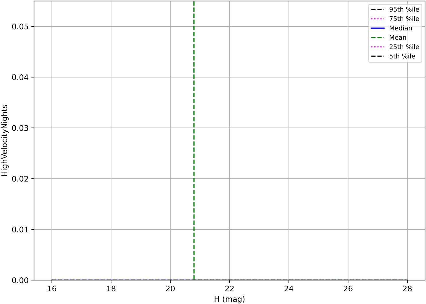
too_elab_r128_d3_griz_v3.4_10yrs: Vatira High velocity pair detection loss
