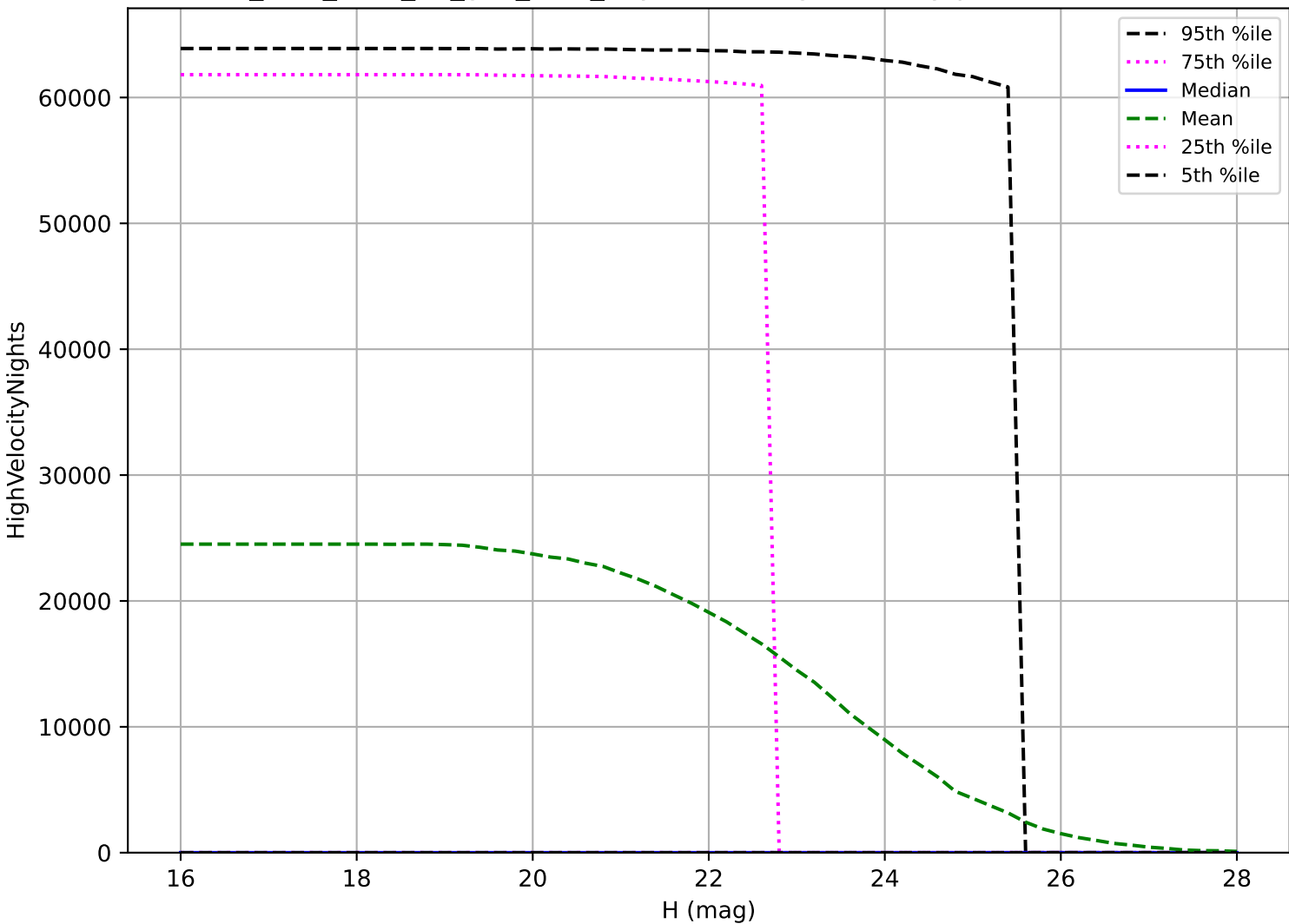
too_elab_r128_d3_griz_v3.4_10yrs: PHA High velocity pair detection loss
