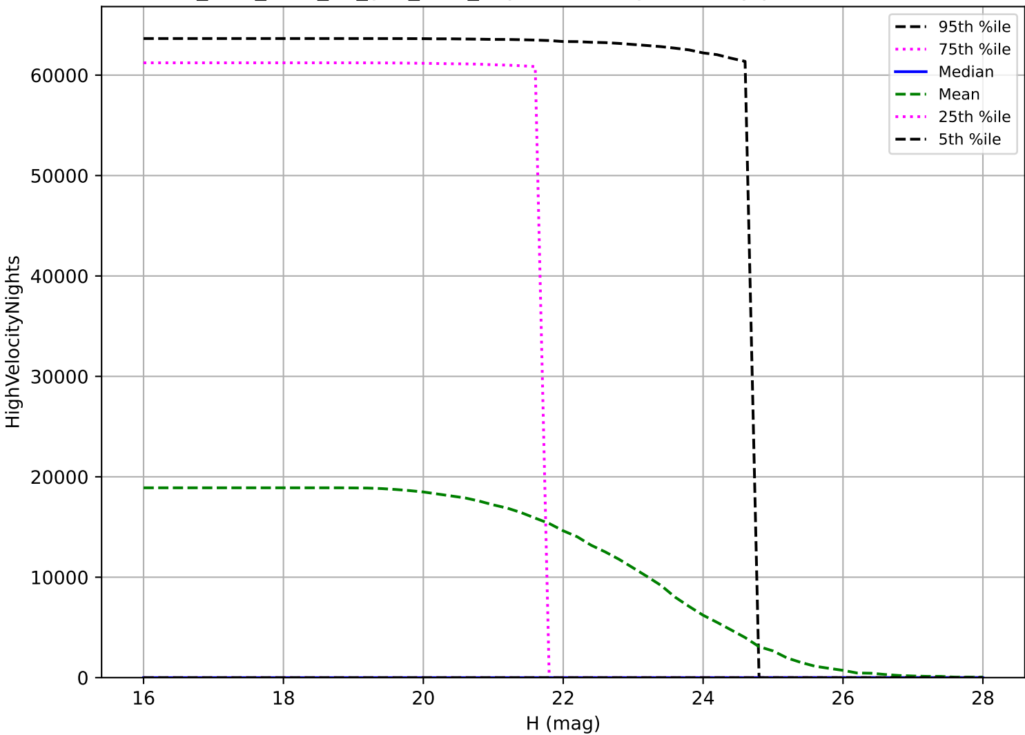
too_elab_r128_d3_griz_v3.4_10yrs: NEO High velocity pair detection loss
