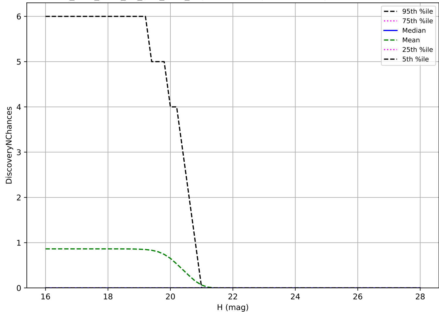
too_elab_r128_d3_griz_v3.4_10yrs: Vatira 3 pairs in 15 nights detection loss
