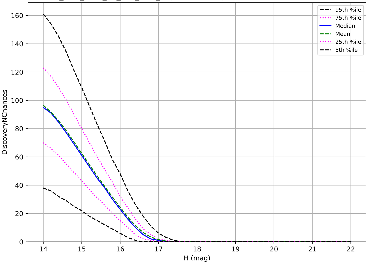
too_elab_r128_d3_griz_v3.4_10yrs: Trojan 3 pairs in 15 nights detection loss
