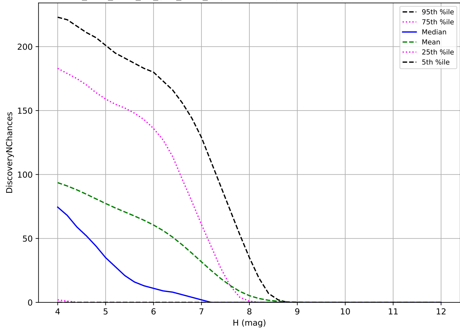
too_elab_r128_d3_griz_v3.4_10yrs: TNO 3 pairs in 15 nights detection loss
