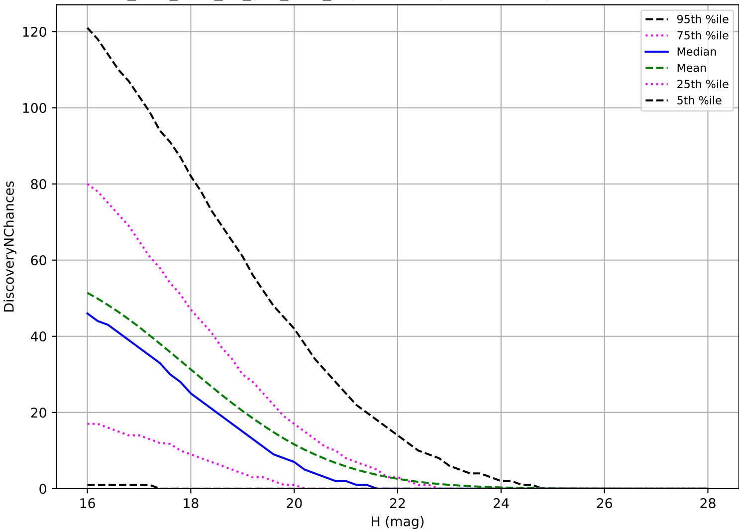
too_elab_r128_d3_griz_v3.4_10yrs: PHA 3 pairs in 15 nights detection loss
