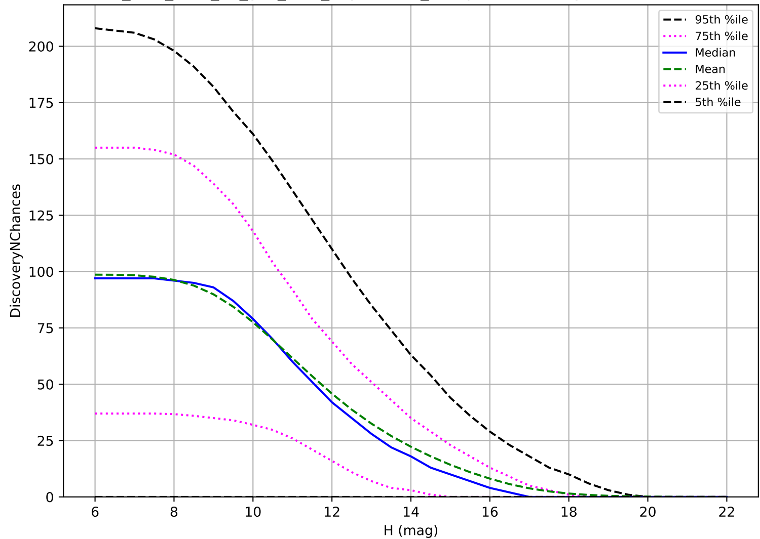
too_elab_r128_d3_griz_v3.4_10yrs: OCC_r5 3 pairs in 15 nights detection loss
