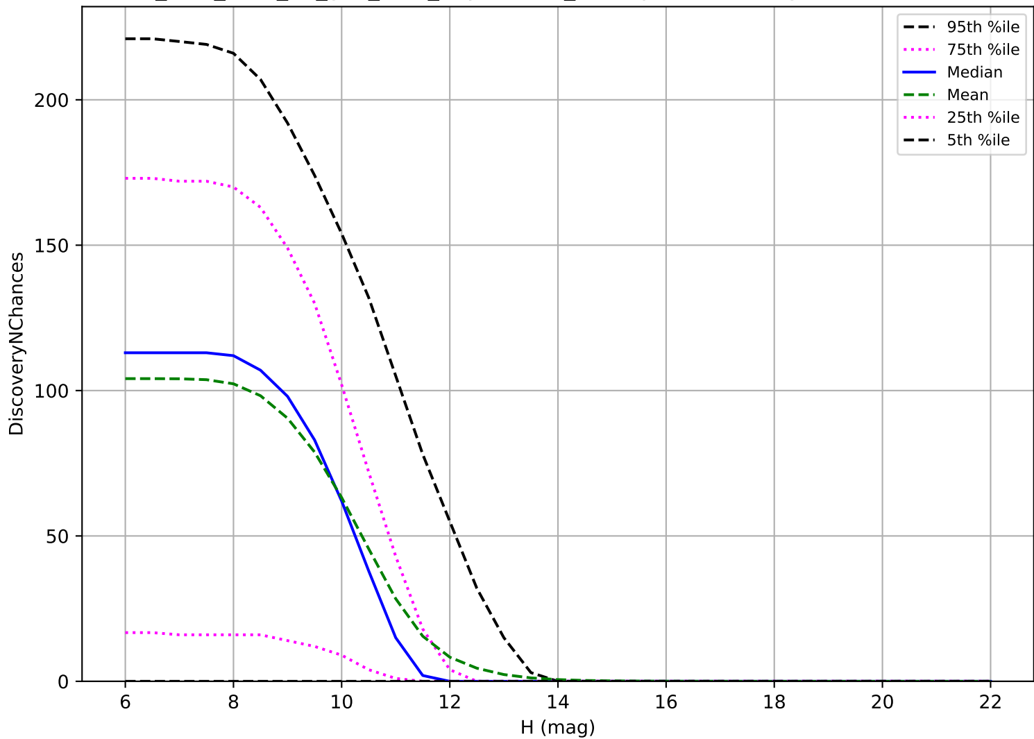
too_elab_r128_d3_griz_v3.4_10yrs: OCC_r20 3 pairs in 15 nights detection loss
