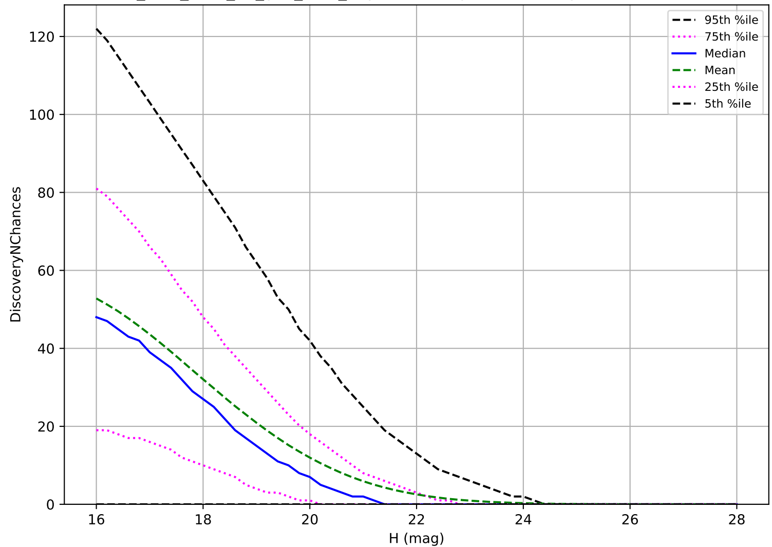
too_elab_r128_d3_griz_v3.4_10yrs: NEO 3 pairs in 15 nights detection loss
