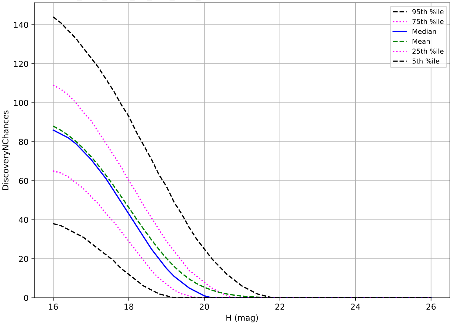
too_elab_r128_d3_griz_v3.4_10yrs: MBA 3 pairs in 15 nights detection loss
