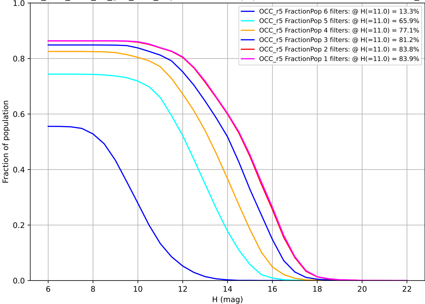
too_elab_r128_d3_griz_v3.4_10yrs: Fraction of population with colors in X filters OCC_r5
