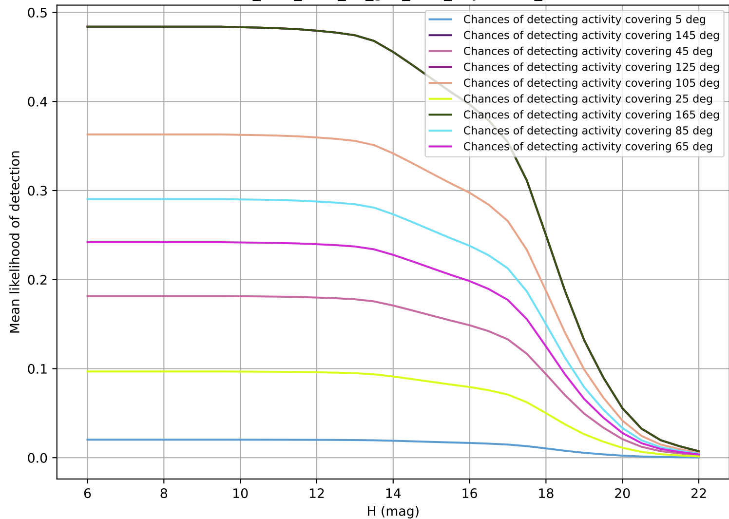
too_elab_r128_d3_griz_v3.4_10yrs OCC_r5
