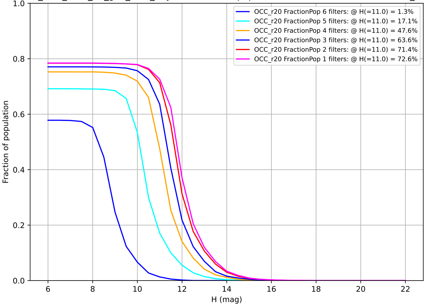
too_elab_r128_d3_griz_v3.4_10yrs: Fraction of population with colors in X filters OCC_r20
